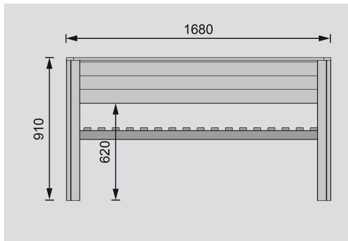
Front (in mm)
